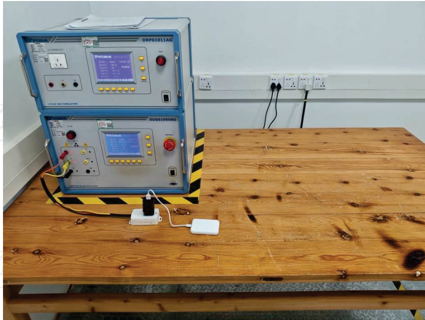
Surge immunity test view
