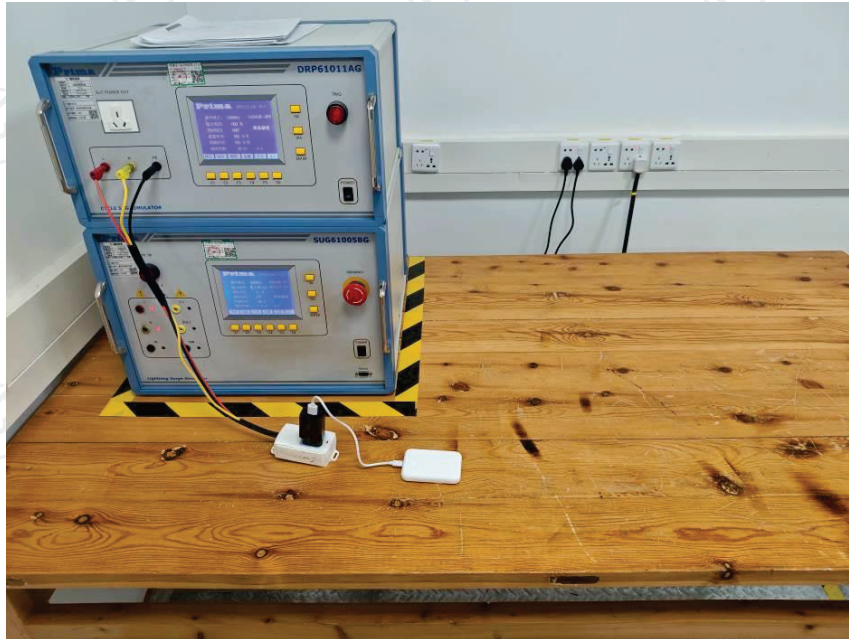
Voltage dips, short interruptions and voltage variations immunity (DIPS) test view
