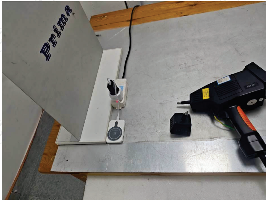
Electrostatic discharge immunity (ESD) test view
