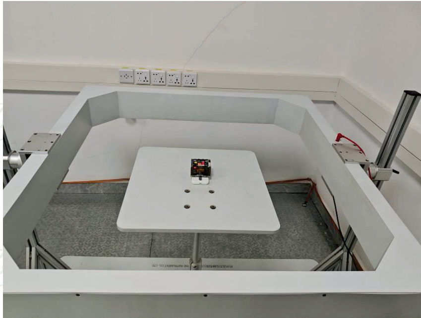
Power frequency magnetic field immunity (PFMF) test view
