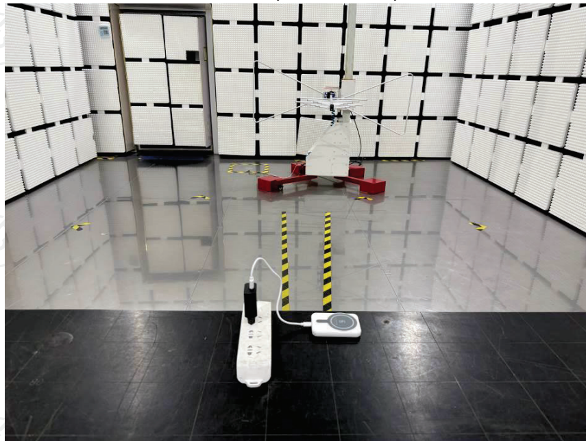
Radiated emission (30 MHz-1 GHz) test view
